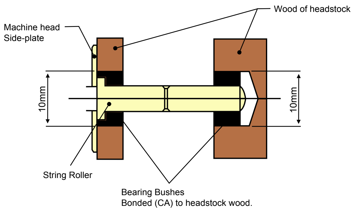
Cross-section of headstock string roller assembly. Showing bearing bushes inside headstock.
